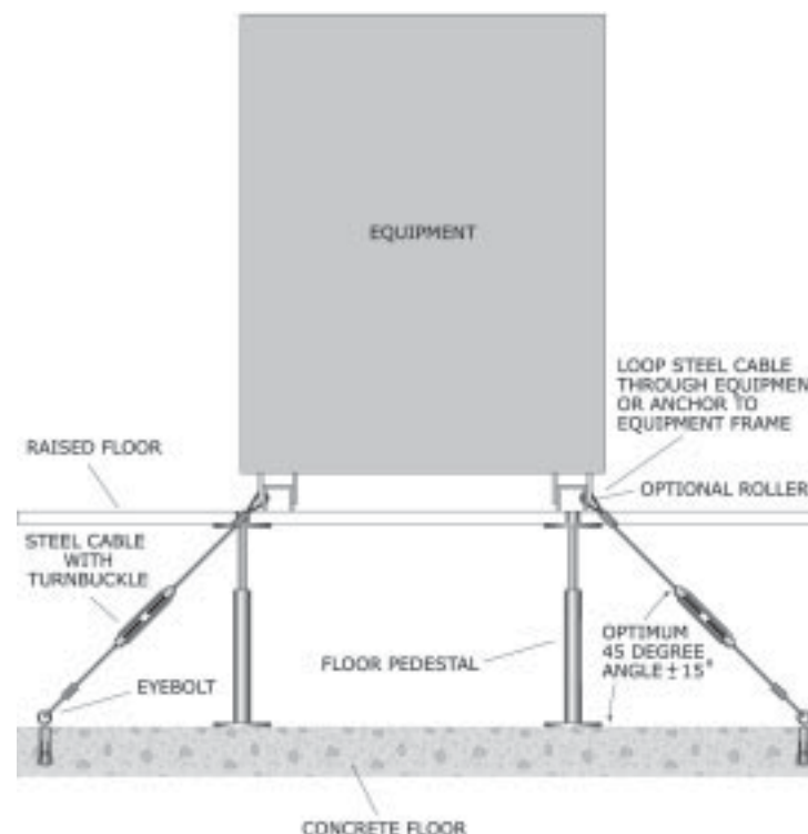
Figure 85: Equipment attached to cables beneath a raised floor.
