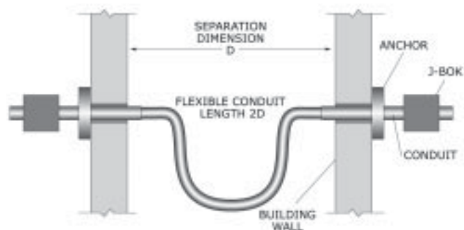
Figure 72: Seismic joint.
