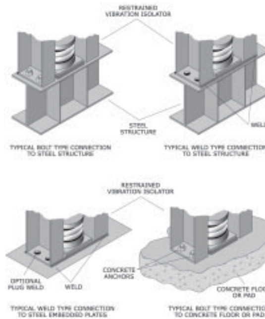
Figure 118: Attachment of restrained vibration isolators to the building structure.
