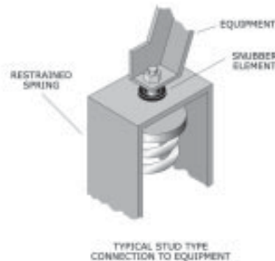
Figure 119: Attachment of equipment to restrained vibration isolators.
