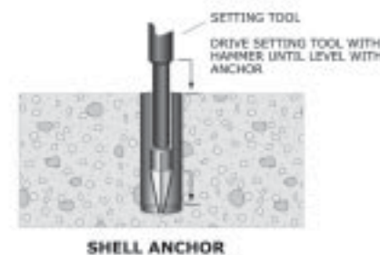
Figure 132: Set shell anchors.
