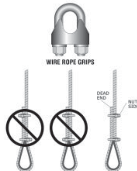
Figure 153: Wire rope grip assemblies.
