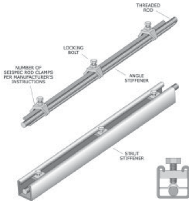
Figure 99: Rod stiffeners.
